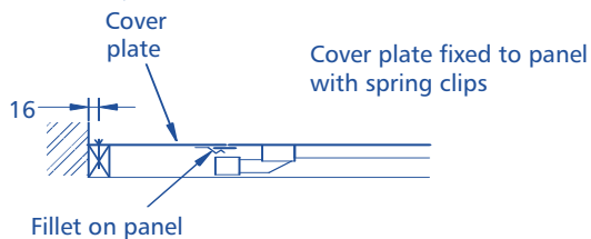
Cover Plate Detail
