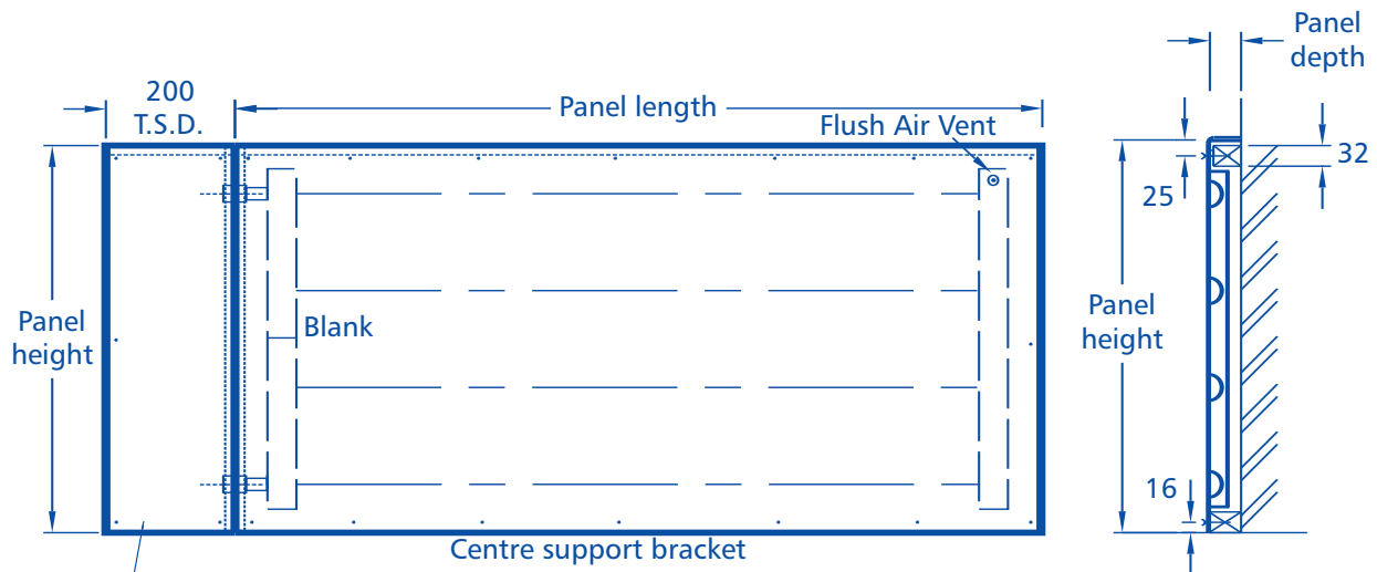
Front Elevation
