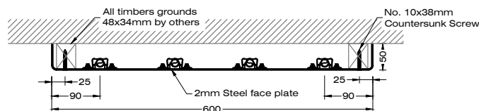
2 Rolled Side Panel Section Detail
