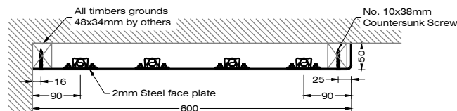
1 Rolled Side Panel Section Detail
