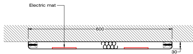
Section View
