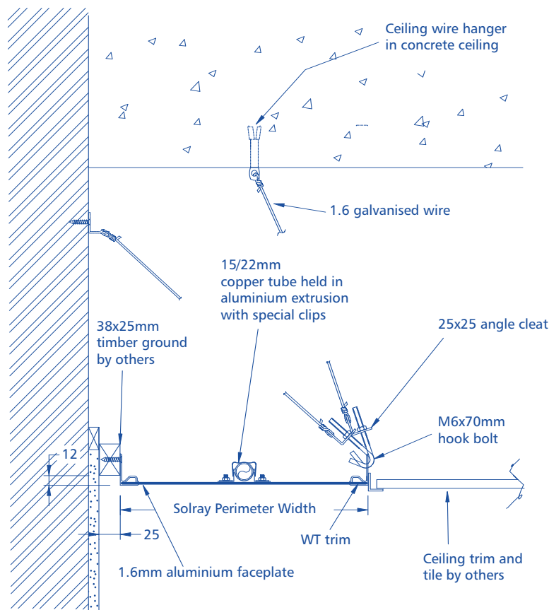
Typical Section Detail
